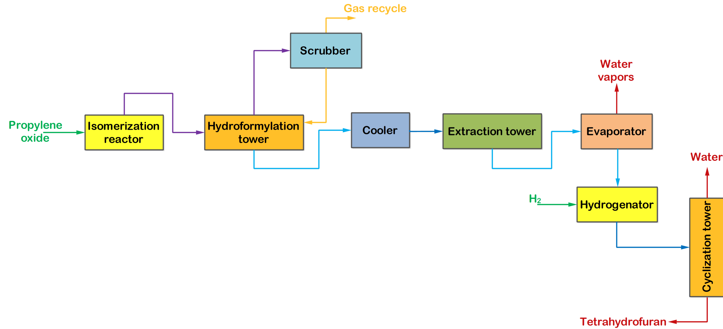
Figure: Manufacture of tetrahydrofuran from propylene oxide
